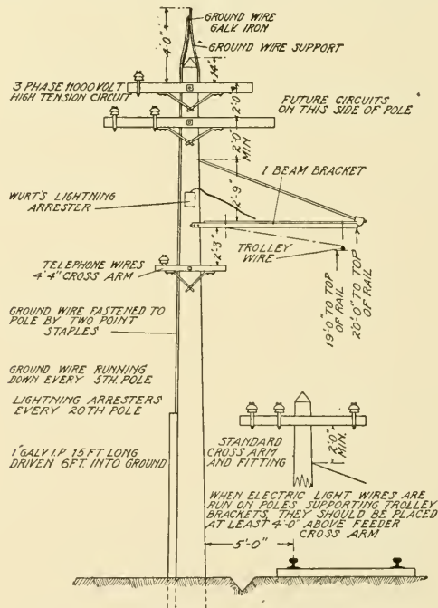
Fig. 197. Catenary Line Construction, Messenger Wire Being Strung on Bracket
